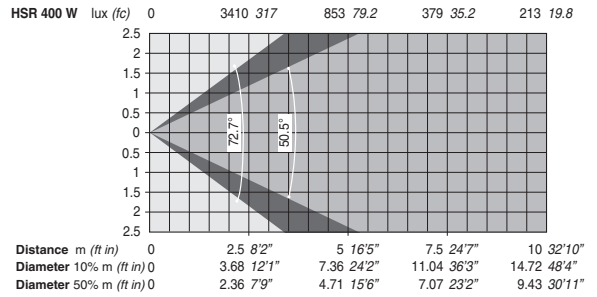
With optional diffusion filter (72.7° 10% - 50.5° 50%)
