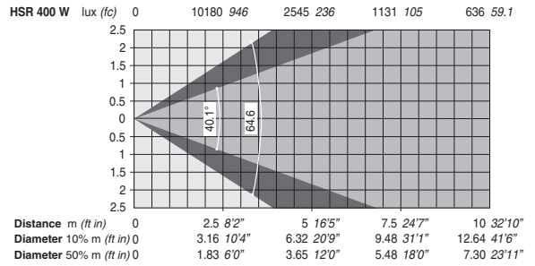
With optional ovalizer filter (X-axis) (64.6° 10% - 40.1° 50%)
